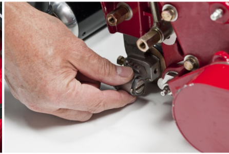
Step 2 - unclip the balljoint
